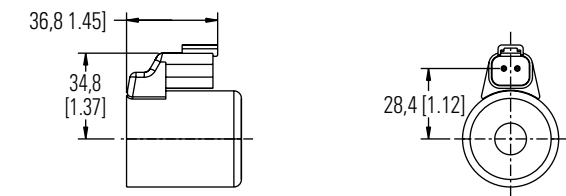
N0 Deutsch Male DTO4-2P integrated connector
