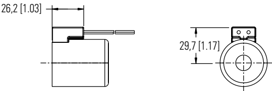
W0 Leadwire
